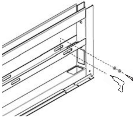
Figure G2 (Drilling assembly)
