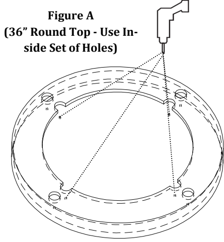
Figure A (36" Round Top - Use In- side Set of Holes) Bottom Side of 36" Round Shown (Outside Hole Set—Glass Kits) (Inside Hole Set—Solid Surface Kits)
